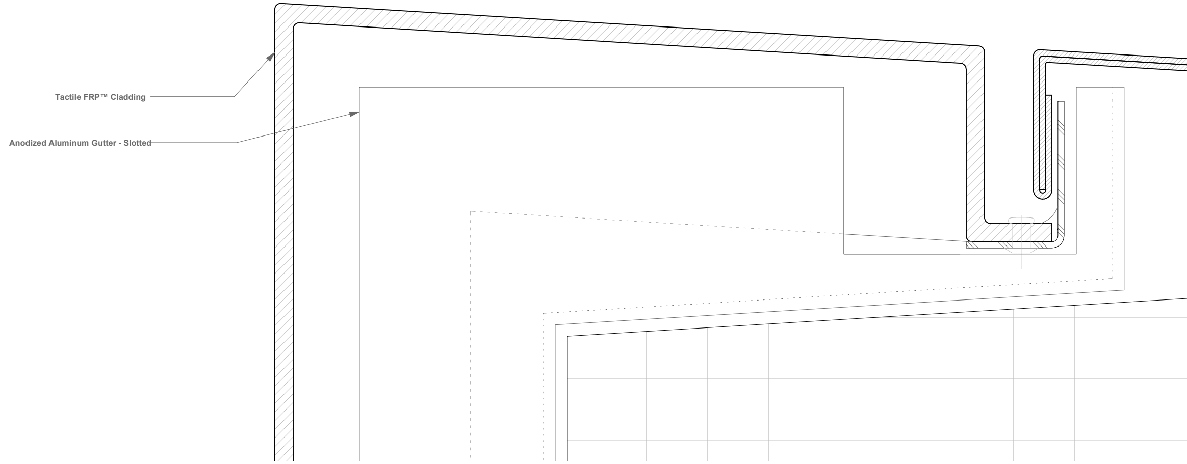
1 Section - Parapet Return Detail - Tactile FRP™ M-04 Scale: Full Scale
