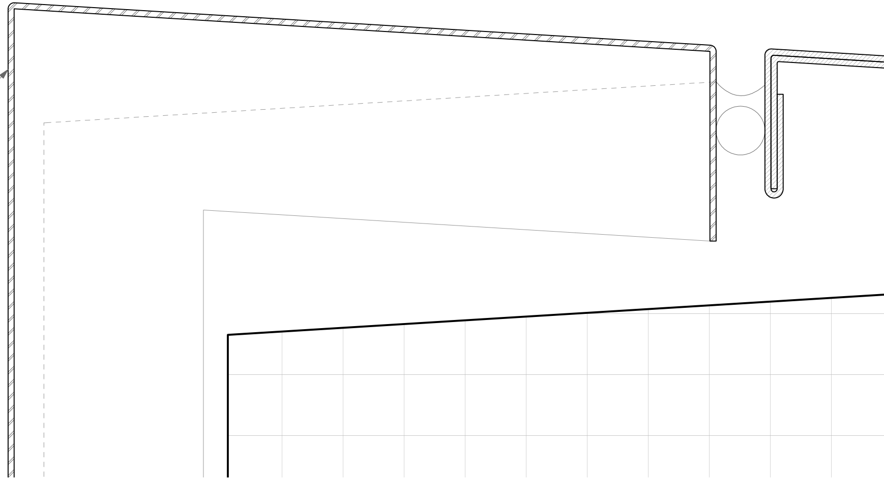
1 Section - Parapet Return Detail - Tactile Porcelain Enamel™ Metal Cladding M-04 Scale: Full Scale
