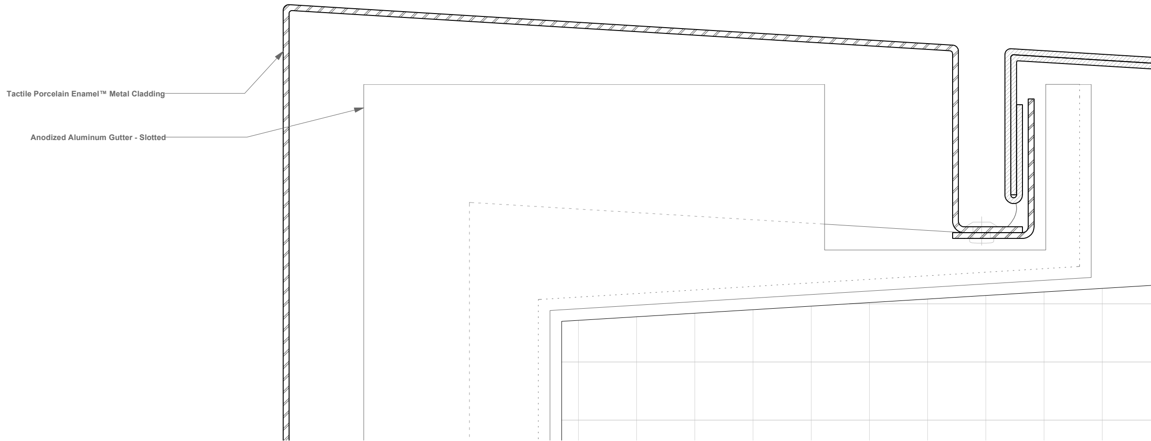
1 Section - Parapet Return Detail - Tactile Porcelain Enamel™ Metal Cladding M-04 Scale: Full Scale
